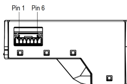
Figure 3 Pin layout. The communication interface connector (ACES 51451-0060N-001) is located at the side of the sensor adjacent to the air outlet.
