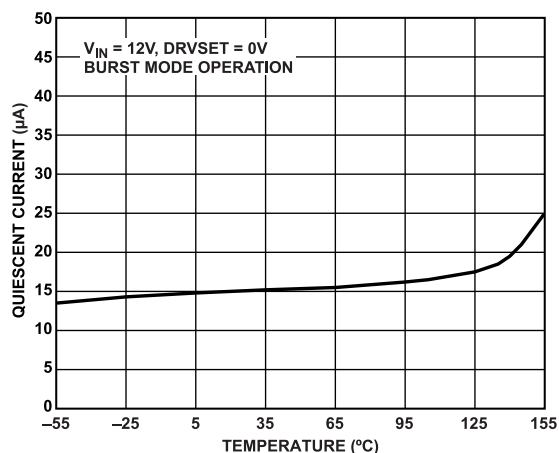
Figure 18. Quiescent Current vs. Temperature
