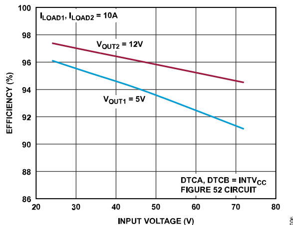
Figure 6. Efficiency vs. Input Voltage ( I_{LOAD1} , I_{LOAD2} Are Load Currents)
