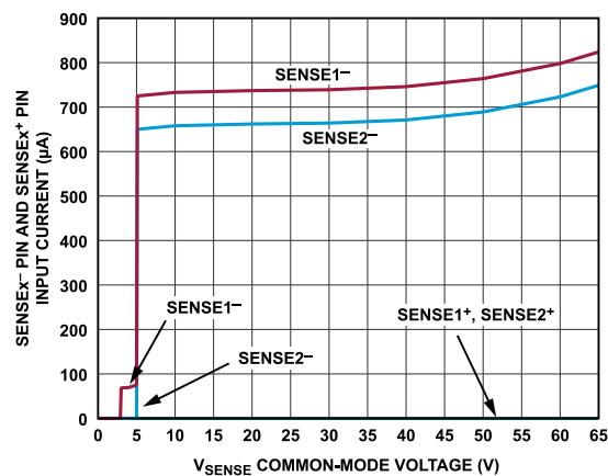
Figure 15. SENSEx Pin and SENSEx^* Pin Input Current vs. V_{SENSE} Common-Mode Voltage
