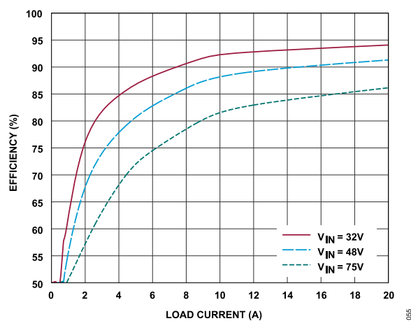
Figure 55. V_{OUT} Efficiency vs. Load Current for Figure 54
