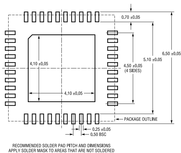
Figure 60. 40-Lead Plastic Side Wettable QFN 6 mm × 6 mm (05-08-1681) Dimensions shown in millimeters
