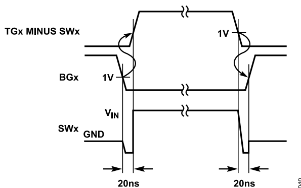
Figure 40. DTCx Pins Tied to GND—Adaptive Dead Time Control
