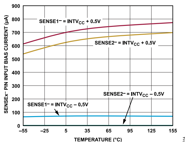
Figure 14. SENSEx Pin Input Bias Current vs. Temperature
