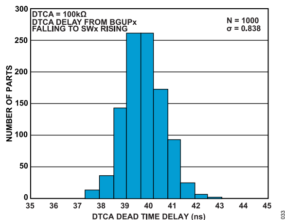
Figure 33. DTCA = 100 kΩ Dead Time Delay Histogram
