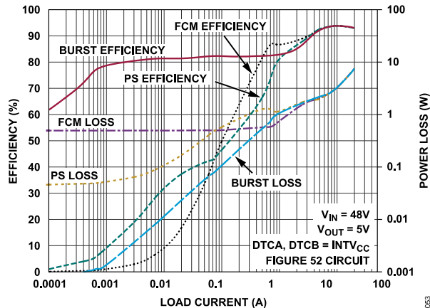
Figure 53. V_{OUT1} Efficiency and Power Loss vs. Load Current for Figure 52
