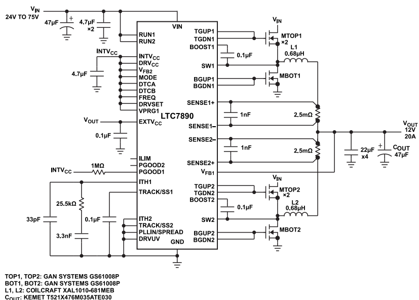
Figure 54. 2-Phase Single Output 12 V_{OUT} , 20 A, 2.25 MHz, Step-Down Regulator Using GaN FETs
