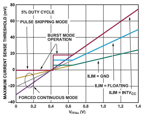
Figure 13. Maximum Current Sense Threshold vs. V_{ITHx}
