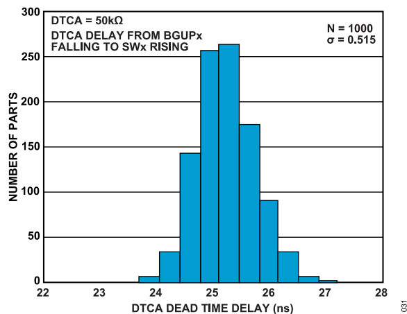
Figure 31. DTCA = 50 kΩ Dead Time Delay Histogram
