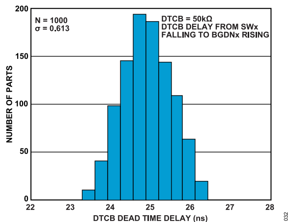
Figure 32. DTCB = 50 kΩ Dead Time Delay Histogram
