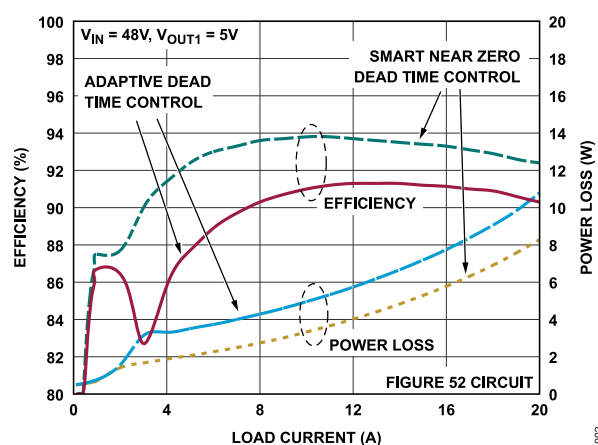
Figure 2. Efficiency and Power Loss vs. Load Current
