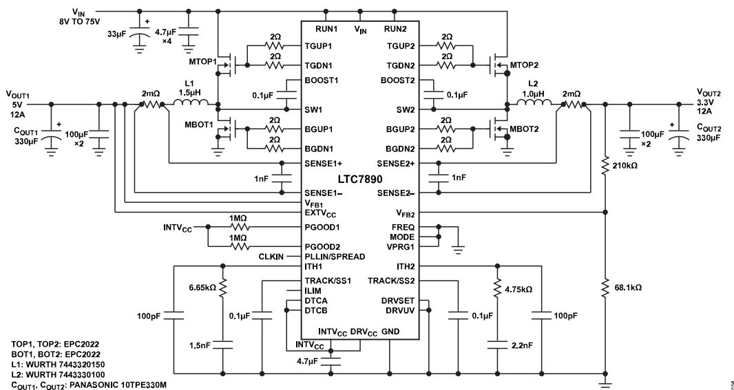
Figure 58. High Efficiency, Dual 5 V/3.3 V, Step-Down Regulator Using GaN FETs
