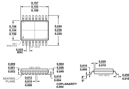
Figure 26. 16-Lead Standard Small Outline Package [SOIC_W] Wide Body (RW-16) Dimensions shown in millimeters and (inches)
