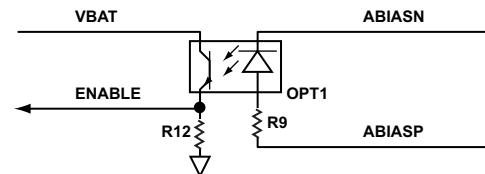
Figure 38. Optional Power Supply Enable Circuit with Optocoupler
