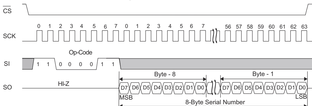
Figure 23. RDSN Instruction
