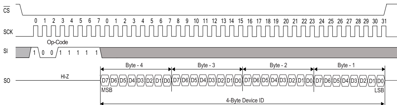
Figure 25. RDID instruction
