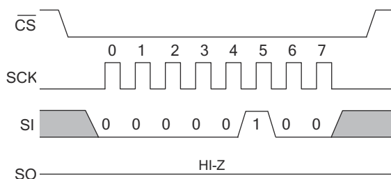
Figure 11. WRDI Instruction
