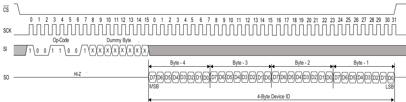
Figure 26. FAST_RDID instruction
