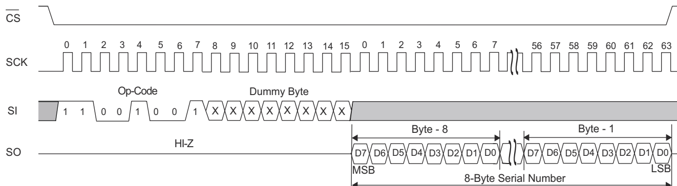
Figure 24. FAST_RDSN Instruction
