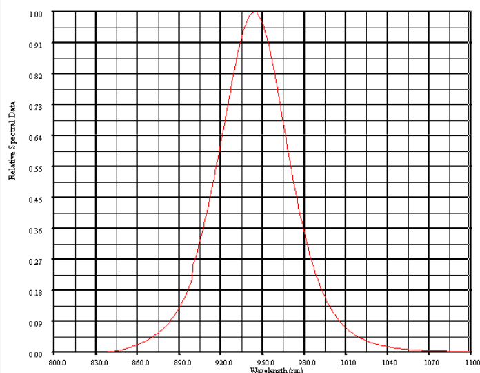
EMITTER SPECTRAL RESPONSE
